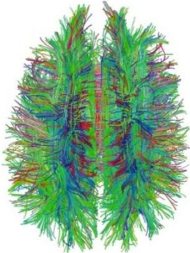
fiber connectome
