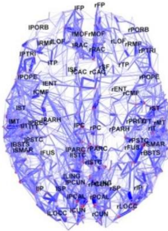
structural connectome
