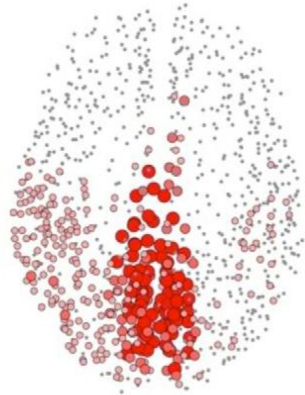
core hubs
